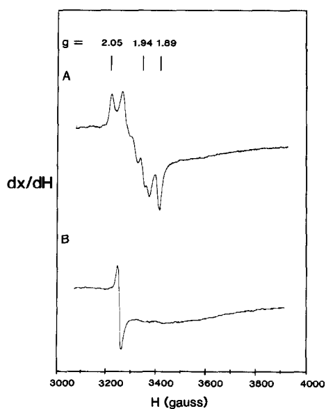
Fig.2. X-band ESR spectrum of F_A and F_B in control (A) and 6.8 M urea-treated, ultracentrifuged (B) PS I reaction centers. Both samples were prepared by addition of 1 mM sodium dithionite and 10 \mu M methyl viologen in 0.1 M glycine, pH 10.0. There was no significant increase in the amount of F_A or F_B upon illumination of the sample at 12 K. Spectrometer conditions: temperature, 12 K; microwave power, 10 mW; microwave frequency, 9.18 GHz; receiver gain, 5.0 \times 10^3 ; modulation amplitude, 10 G at 100 kHz.
